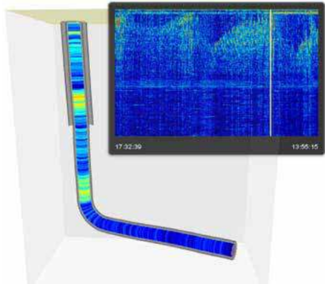
Real-time visualization of in-well flow regimes using DAS
